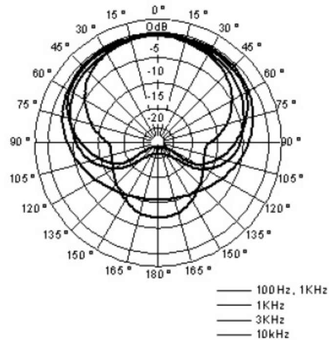
Directivity Characteristics
