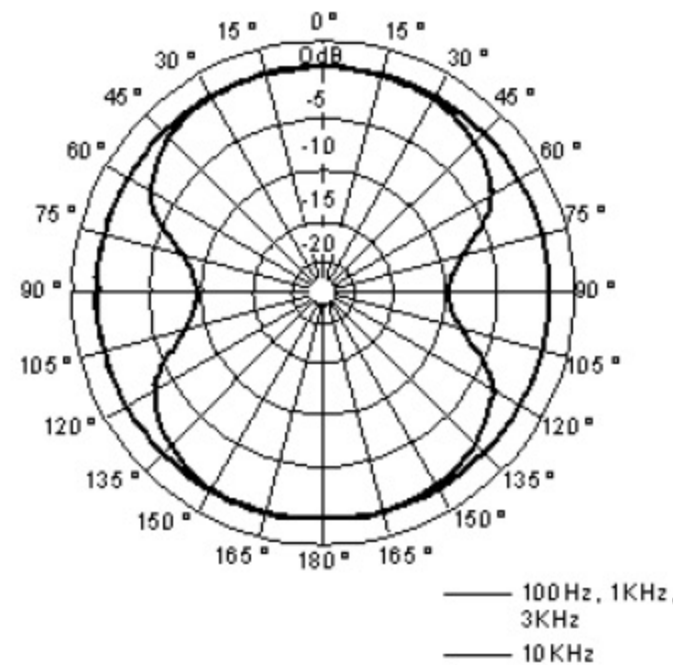
Directivity Characteristics
