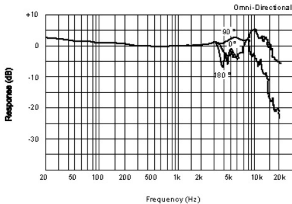
Frequency Response Characteristics
